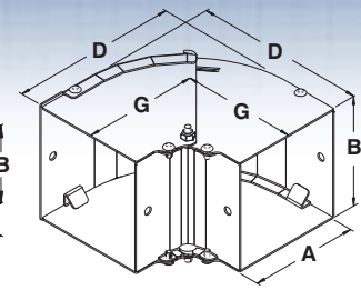
Coude ajustable 19° to 48° et Coude ajustable 42° to 93°
